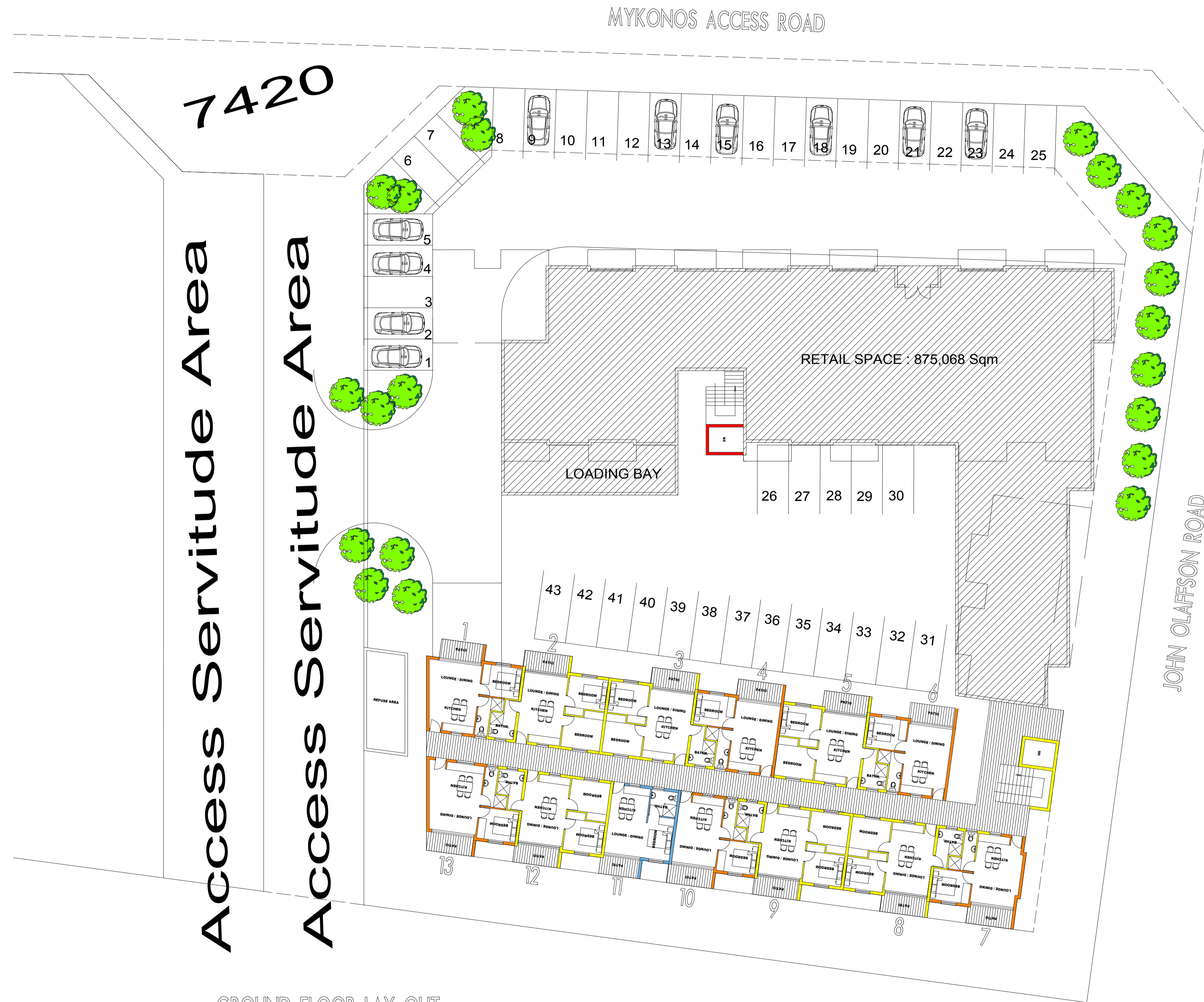
GROUND FLOOR LAY OUT 1 : 200
