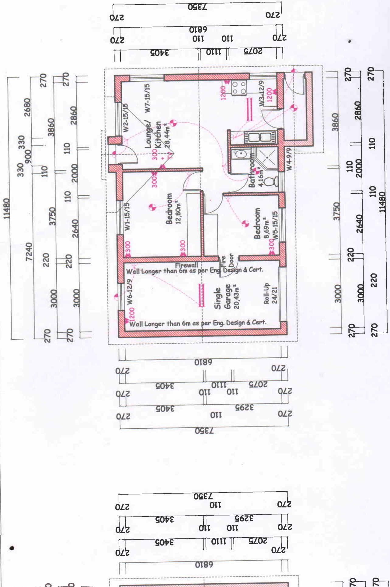
Typical 2 Bedroom Units 11, 12 & 13 Floorplan Scale 1:100
